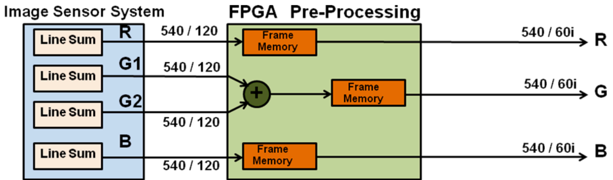
Figure 11 The 540-line fields for the interlaced 1080@60i format are structured within the image sensor readout process which occurs at 120fps to reduce the rolling shutter effect
