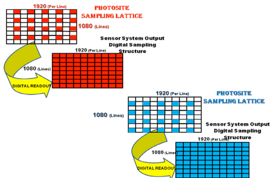
Figure 6 Showing the Red and Blue sensor readout that structures the sparsely-sampled Photosites into the standardized output digital video sampling structure
